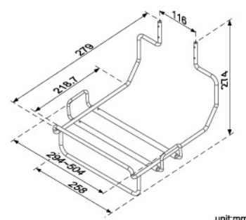
HAA-11 Keyboard Tray
